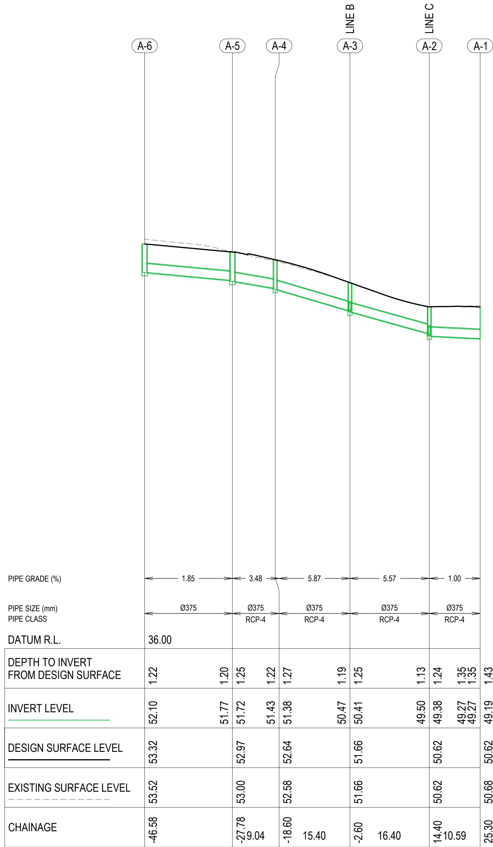
LINE A A1 HORIZONTAL SCALE 1 : 500 A1 VERTICAL SCALE 1 : 100
